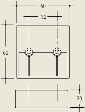
724 1000 Kg Carico max- Max load 60x60 h 20 i 32 VE | VS | VG | VM | MT | KU | SP
