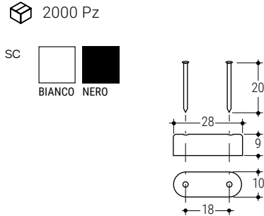
112 p Fermaporte con chiodi montati o smontati - piccolo Door-fastener with mounted or mounted nails - small
