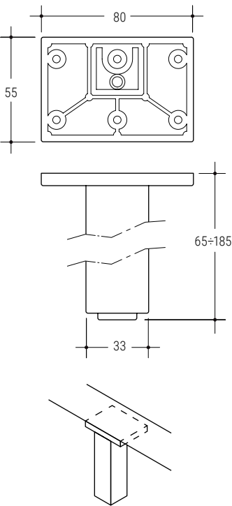
Piedino intermedio Intermediate foot
