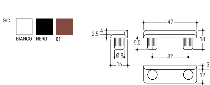
189 Fermaporte con 2 spine Door fastener with 2 pins
