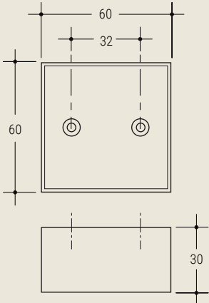
731 1000 Kg Carico max- Max load 60x60 h 30 i 32 VE | VS | VG | MT | KU | SP
