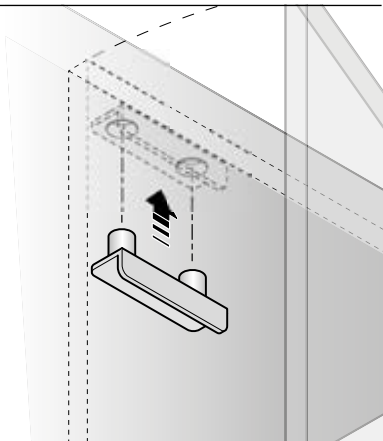
189 Fermaporte con 2 spine Door fastener with 2 pins
