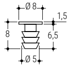
121 D Paracolpo morbido testa liscia Soft bumper with smooth head 5000 Pz
