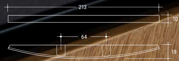
307 213x10 p 19 i 64 VE | VS | VG | VR | KU | SP
