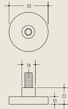
709B 290 Kg Carico max- Max load Ø 52 h 22 v. 10MA VE | VS | VG | VM | MT | SP
