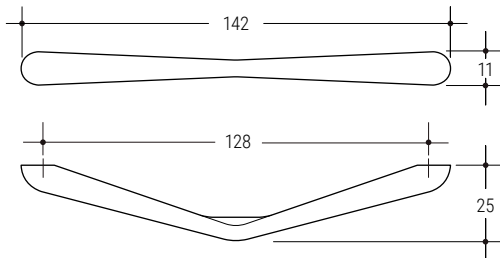
374C 142x11 p 25 i 128 VE | VS | VG | VM | VR | GA | KU | SP
