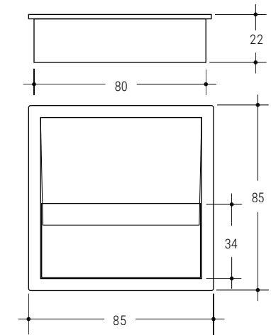
1626 85x85 h 22 VE | VS | VG | MT | GA | SP
