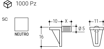
176 B Reggipiano in nylon Nylon plane bracket
