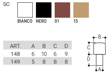
148-149 Reggipiano Elastic plane bracket
