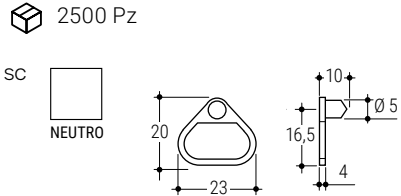
176 A Fermapiano elastico h 20 Elastic bracket fastener h 20
