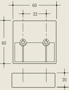
724 1000 Kg Carico max- Max load 60x60 h 20 i 32 VE | VS | VG | VM | MT | KU | SP
