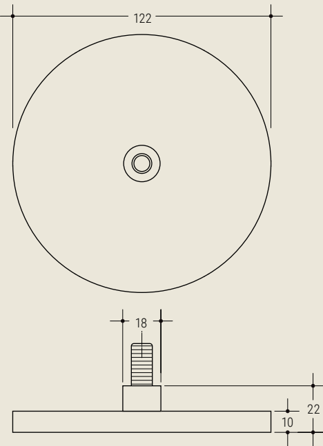
715 290 Kg Carico max- Max load Ø 122 h 22 v. 10MA VE | VS | VG | VM | MT | SP
