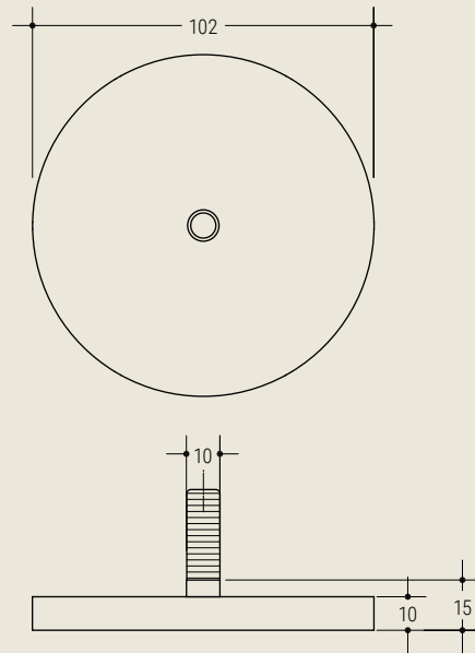
714 290 Kg Carico max- Max load Ø 102 h 15 v. 10MA VE | VS | VG | VM | MT | SP
