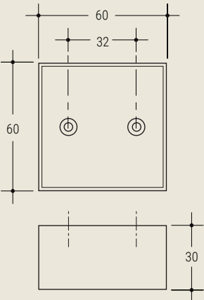
731 1000 Kg Carico max- Max load 60x60 h 30 i 32 VE | VS | VG | MT | KU | SP
