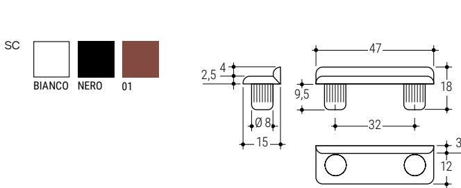
189 Fermaporte con 2 spine Door fastener with 2 pins
