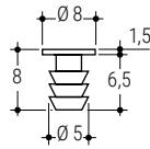
121 D Paracolpo morbido testa liscia Soft bumper with smooth head 5000 Pz
