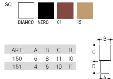
150-151 Reggipiani in nylon Nylon plane brackett
