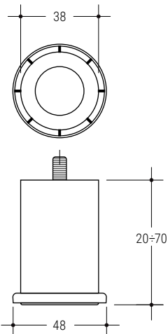
145B Ø 38/48 v. A1-A2-B1-B h 20-25-30-35-40-45-50-55-60-65-70 VE | VS | VG | MT | KU | SP
