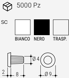
113 A Paracolpo a pressione testa morbida Pressur-shock absorber with soft head
