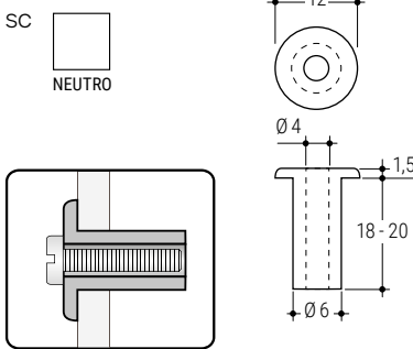
1890 Rondella salva specchi Mirror protecting washer 1000 Pz
