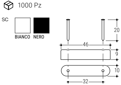
112 G Fermaporte con chiodi montati o smontati - grande. Door-fastener with mounted or mounted nails - large
