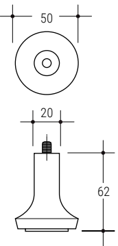
759 Ø 20/50 h 62 v. A2 VE | VG | VM | MT | KU | SP
