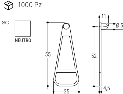
176 C Fermapiano elastico h 55 Elastic bracket fastener h 55
