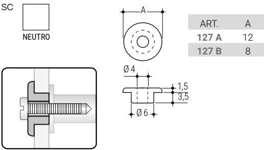
127 A-127 B Rondella salva specchi Mirror protecting washer 10000 Pz
