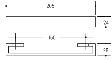
037B 205x24 p 28 i 160 VE | VS | VG | VV | SP | ST - - VE | VS | VG | GA | SP
